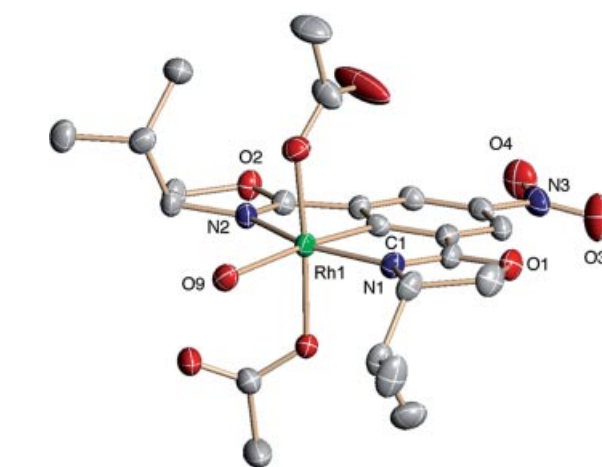
Figure 1. Molecular structure of complex 5a . Selected bond lengths [Å] and angles [°]: \text{Rh1}-\text{C1} 1.914(3), \text{Rh1}-\text{N1} 2.055(3), \text{Rh1}-\text{N2} 2.057(3), \text{Rh1}-\text{O9} 2.195(2); \text{C1}-\text{Rh1}-\text{O9} 174.38(12), \text{N1}-\text{Rh1}-\text{N2} 159.00(10), \text{C1}-\text{Rh1}-\text{N1} 79.72(12), \text{C1}-\text{Rh1}-\text{N2} 79.29(12).
